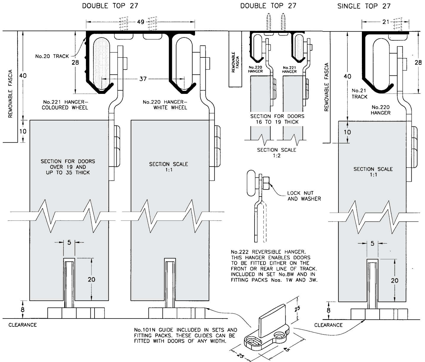
DOUBLE TOP 27 2 DOOR APPLICATION
