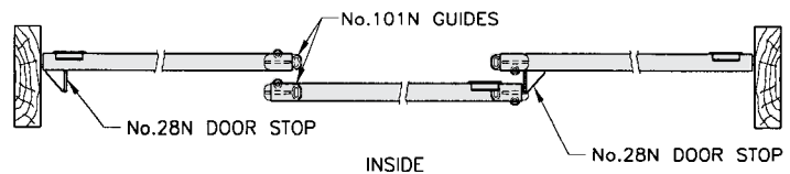
DOUBLE TOP 27 3 DOOR APPLICATION
