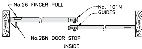
DOUBLE TOP 27 2 DOOR APPLICATION
